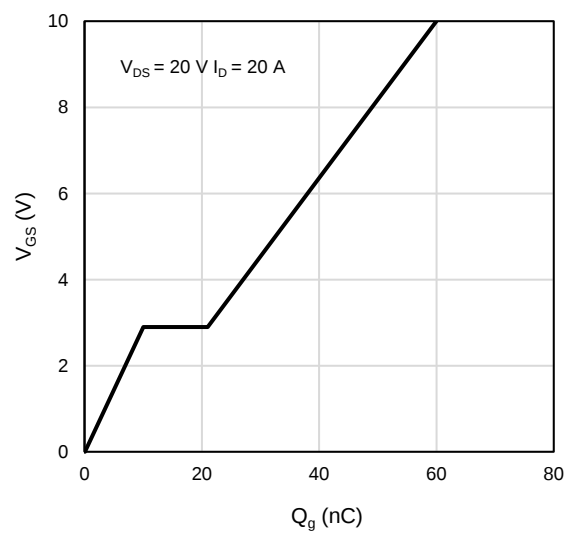
Figure 10: Gate-Charge Characteristics
