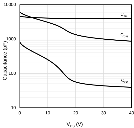
Figure 9: Capacitance Characteristics
