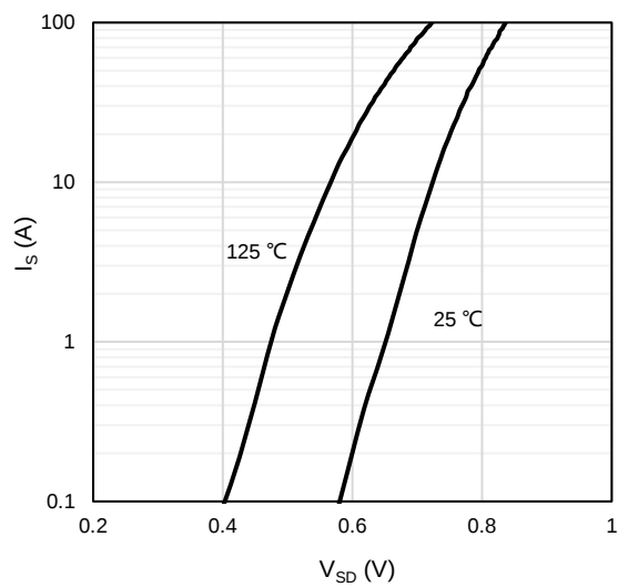
Figure 7: Body-Diode Characteristics
